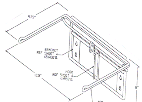
SCANRACK Wall mounted T-Shirt Bag Rack
